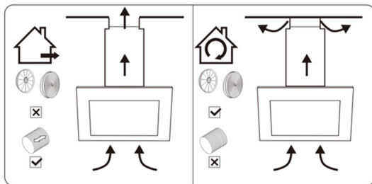
Ducted option
